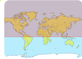
Southern Hemisphere
